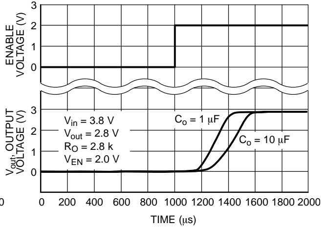
Figure 17. Turn-On Response
