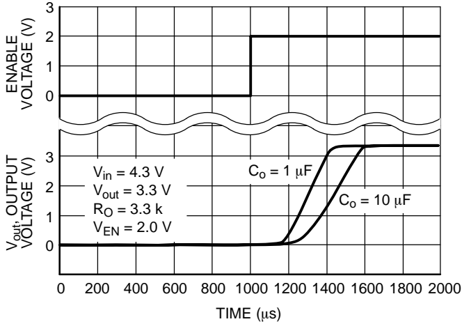
Figure 16. Turn-On Response
