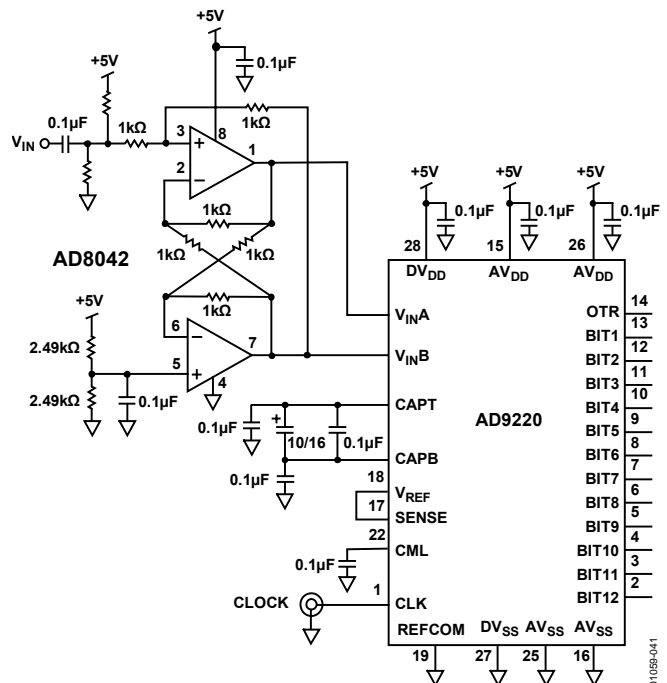
Figure 41. AD8042 Differential Driver for the AD9220 12-Bit, 10-MSPS ADC
