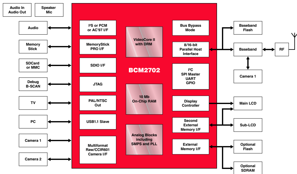
BCM2702 Block Diagram
