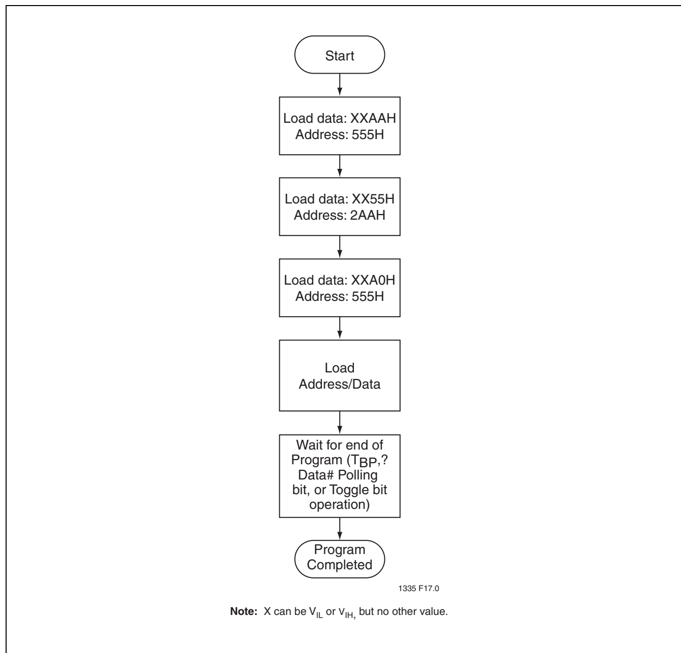
FIGURE 22: Program Algorithm
