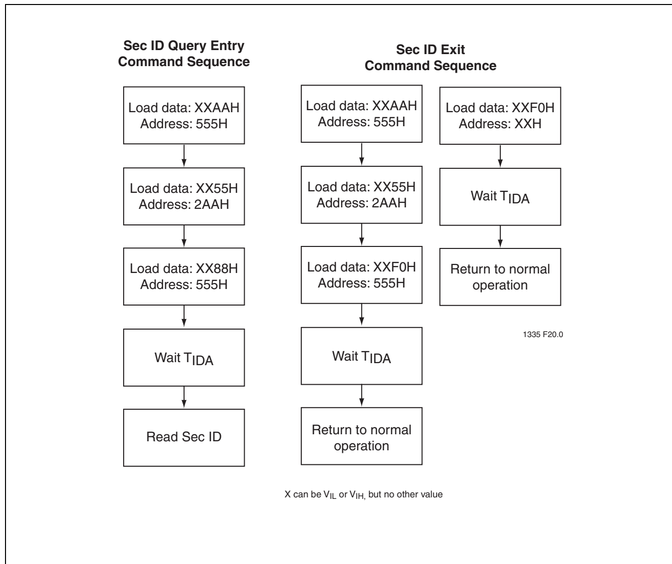
FIGURE 25: Software Sec ID Command Flowcharts
