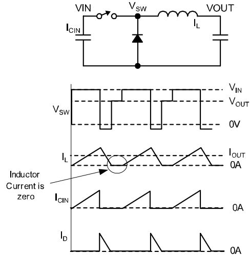
Figure 5. Discontinuous Operation
