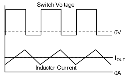
Figure 2. Continuous Operation
