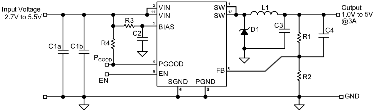
MIC2207 Schematic
