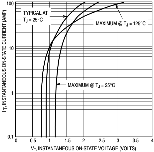
Figure 7. On-State Characteristics
