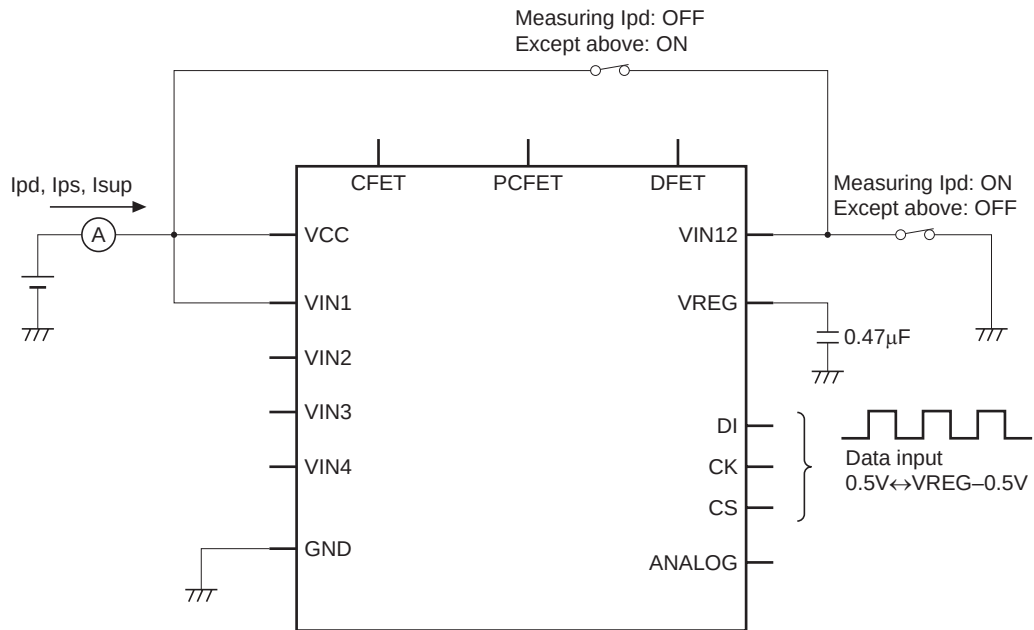
Measurement circuit 1
