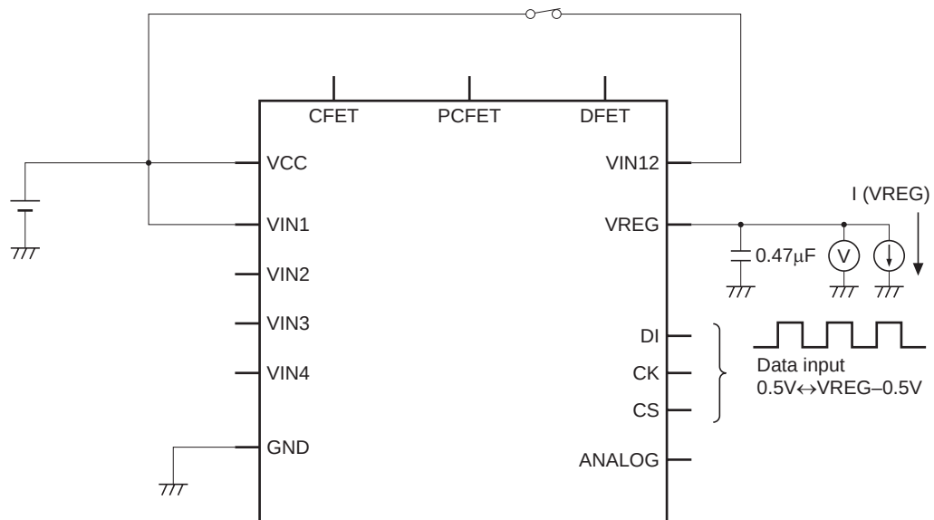
Measurement circuit 2
