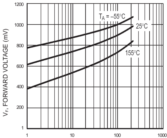
Figure 1. Forward Voltage
