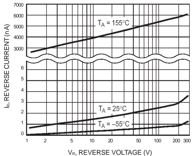
Figure 2. Reverse Leakage
