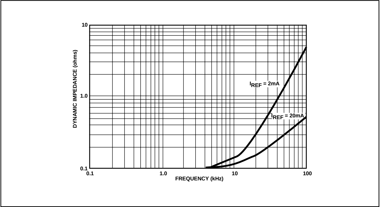
Fig.3 Dynamic impedance
