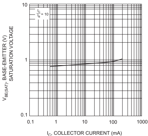
I_C , COLLECTOR CURRENT (mA) Fig. 9, Typical Base-Emitter Saturation Voltage vs. Collector Current (NPN-4124)
