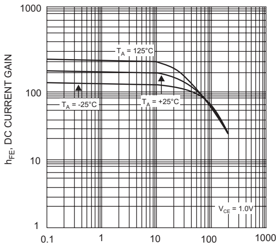
I_C , COLLECTOR CURRENT (mA) Fig. 7, Typical DC Current Gain vs. Collector Current (NPN-4124)
