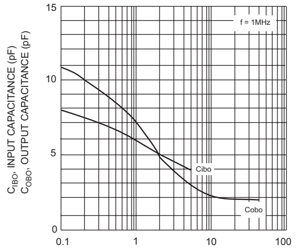
V_{CB} , COLLECTOR-BASE VOLTAGE (V) Fig. 6, Input and Output Capacitance vs. Collector-Base Voltage (NPN-4124)
