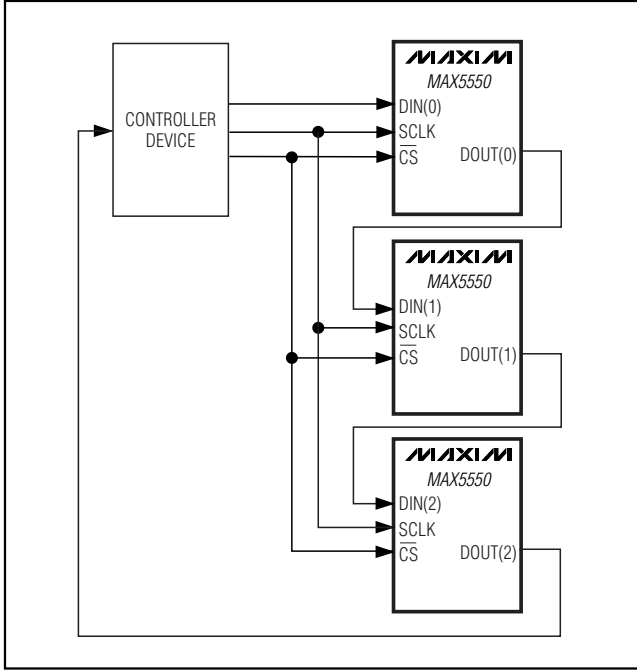
Figure 8. Daisy-Chain Configuration
