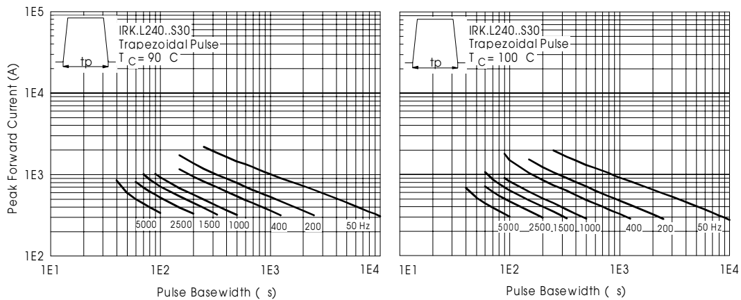
Fig.26-Frequency Characteristics
