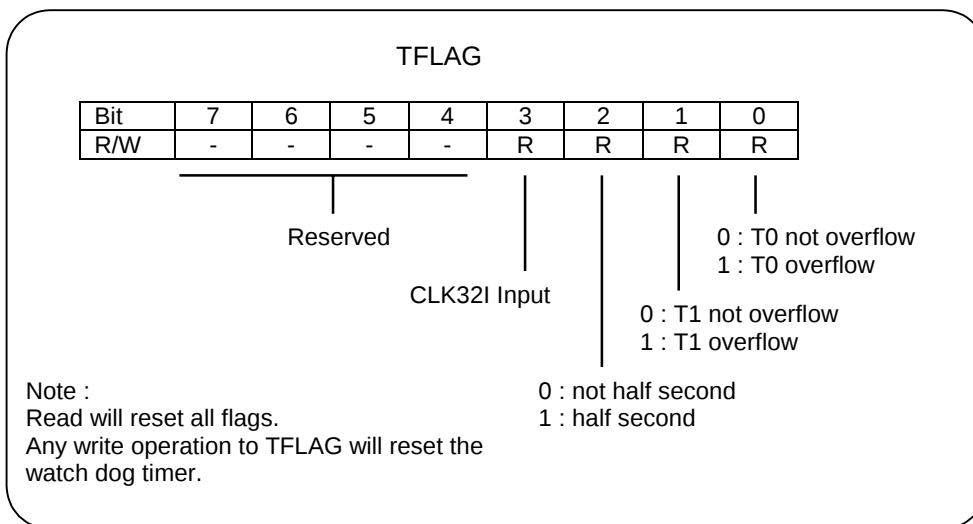
Figure 16. Timer Flag Status Register/Watch-dog Reset
