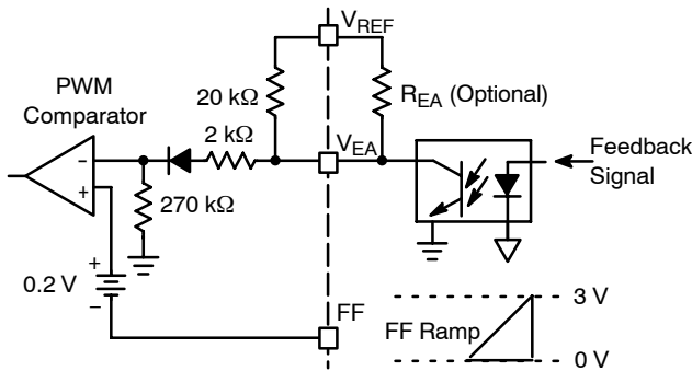
Figure 45. Optocoupler Driving V_{EA} Input
