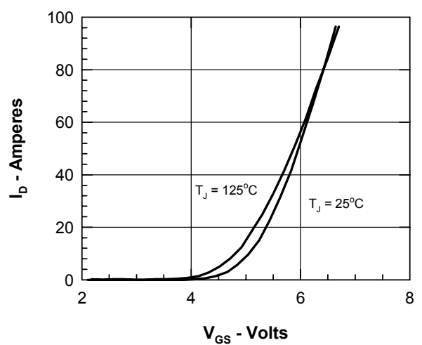
Figure 6. Admittance Curves
