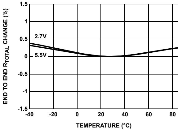
FIGURE 9. END TO END R_{TOTAL} % CHANGE vs TEMPERATURE FOR 50kΩ (W)
