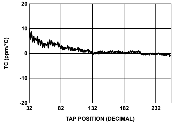
FIGURE 10. TC FOR VOLTAGE DIVIDER MODE IN ppm FOR 50kΩ (W)
