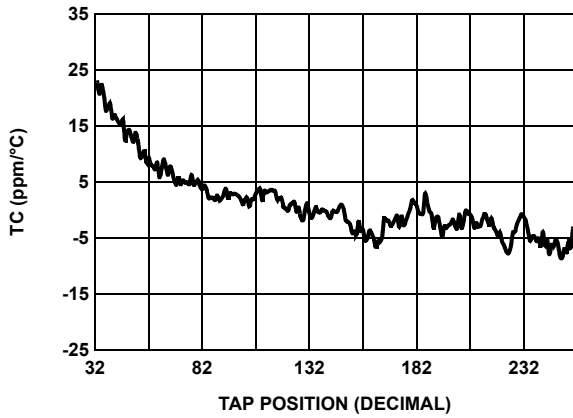
FIGURE 11. TC FOR RHEOSTAT MODE IN ppm FOR 50kΩ (W)
