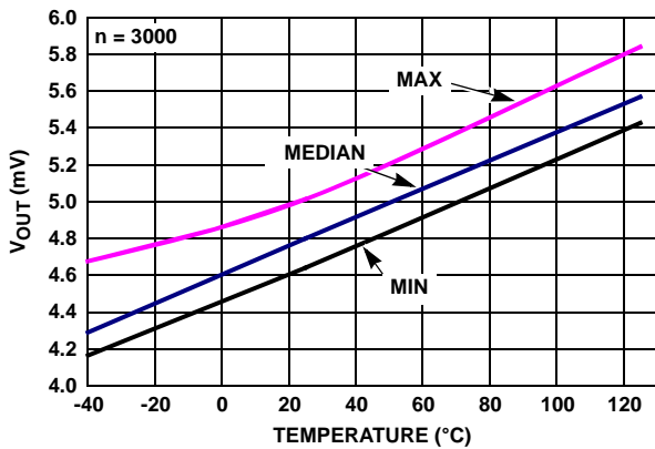
FIGURE 35. ISL28271 V_{OUT} LOW vs TEMPERATURE R_L = 100k , V_S = \pm 2.5V
