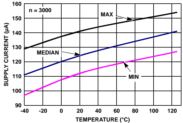
FIGURE 22. ISL28272 SUPPLY CURRENT ENABLED vs TEMPERATURE V_S = \pm 2.5V , V_{IN} = 0V
