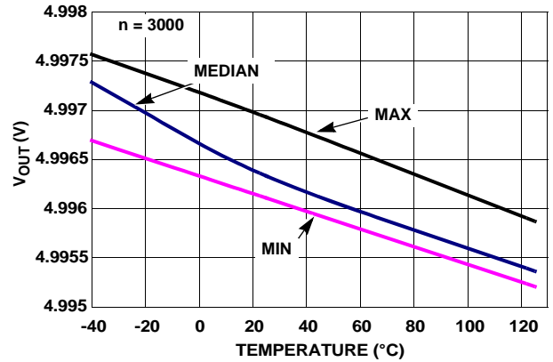
FIGURE 32. ISL28272 V_{OUT} HIGH vs TEMPERATURE R_L = 100k , V_S = \pm 2.5V
