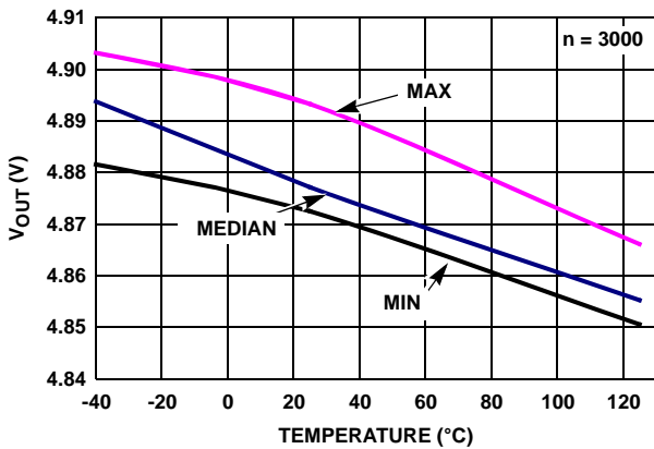
FIGURE 29. ISL28271 V_{OUT} HIGH vs TEMPERATURE R_L = 1k , V_S = \pm 2.5V
