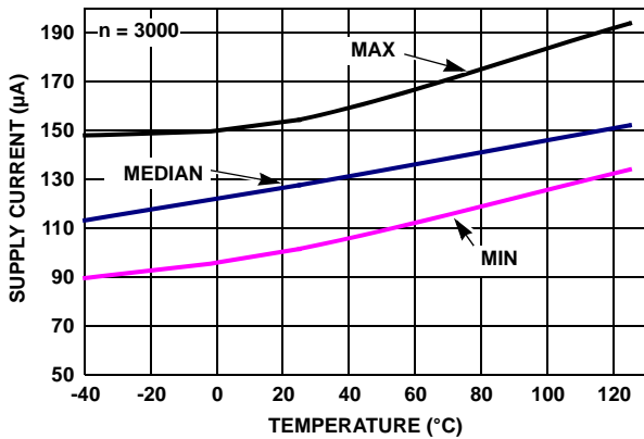
FIGURE 21. ISL28271 SUPPLY CURRENT ENABLED vs TEMPERATURE V_S = \pm 2.5V , V_{IN} = 0V
