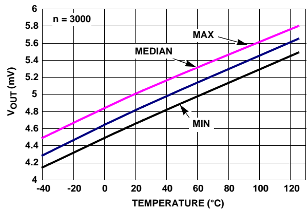
FIGURE 36. ISL28272 V_{OUT} LOW vs TEMPERATURE R_L = 100k , V_S = \pm 2.5V
