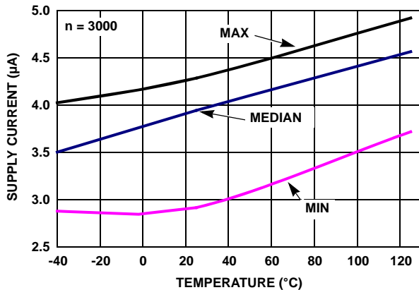
FIGURE 23. ISL28271 SUPPLY CURRENT DISABLED vs TEMPERATURE V_S = \pm 2.5V , V_{IN} = 0V
