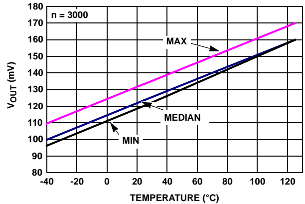
FIGURE 34. ISL28272 V_{OUT} LOW vs TEMPERATURE R_L = 1k , V_S = \pm 2.5V
