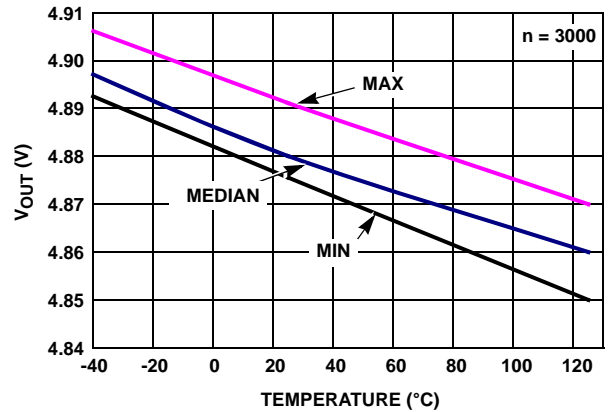
FIGURE 30. ISL28272 V_{OUT} HIGH vs TEMPERATURE R_L = 1k , V_S = \pm 2.5V
