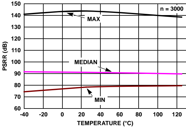
FIGURE 27. ISL28271 PSRR vs TEMPERATURE V_S = \pm 1.2V TO \pm 2.5V
