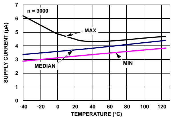
FIGURE 24. ISL28272 SUPPLY CURRENT DISABLED vs TEMPERATURE V_S = \pm 2.5V , V_{IN} = 0V
