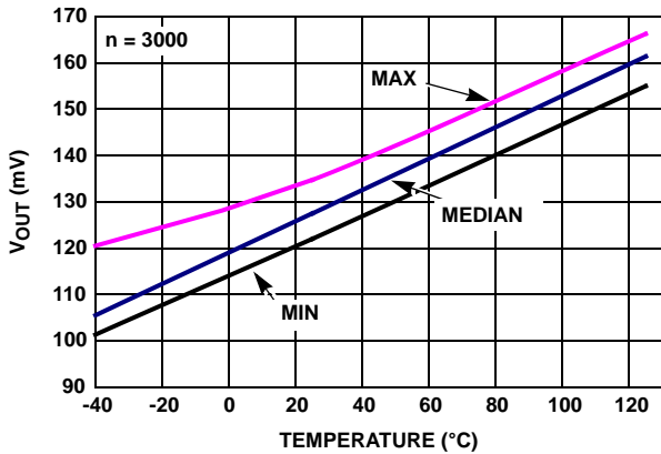
FIGURE 33. ISL28271 V_{OUT} LOW vs TEMPERATURE R_L = 1k , V_S = \pm 2.5V
