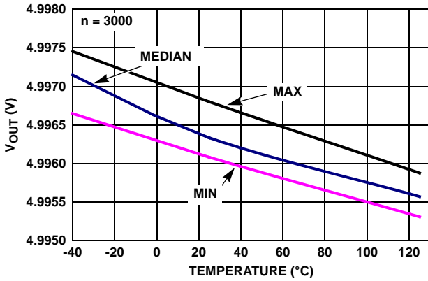
FIGURE 31. ISL28271 V_{OUT} HIGH vs TEMPERATURE R_L = 100k , V_S = \pm 2.5V
