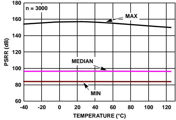
FIGURE 28. ISL28272 PSRR vs TEMPERATURE V_S = \pm 1.2V TO \pm 2.5V
