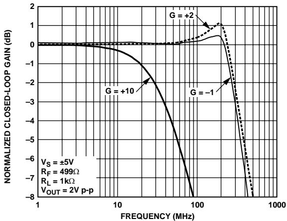
Figure 15. Large Signal Frequency Response for Various Gains
