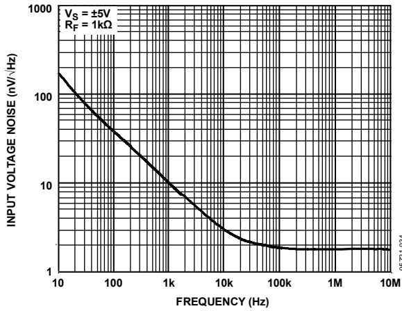
Figure 34. Input Voltage Noise vs. Frequency
