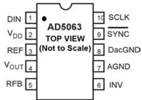
Figure 3. AD5063 10 ld uSOIC.
