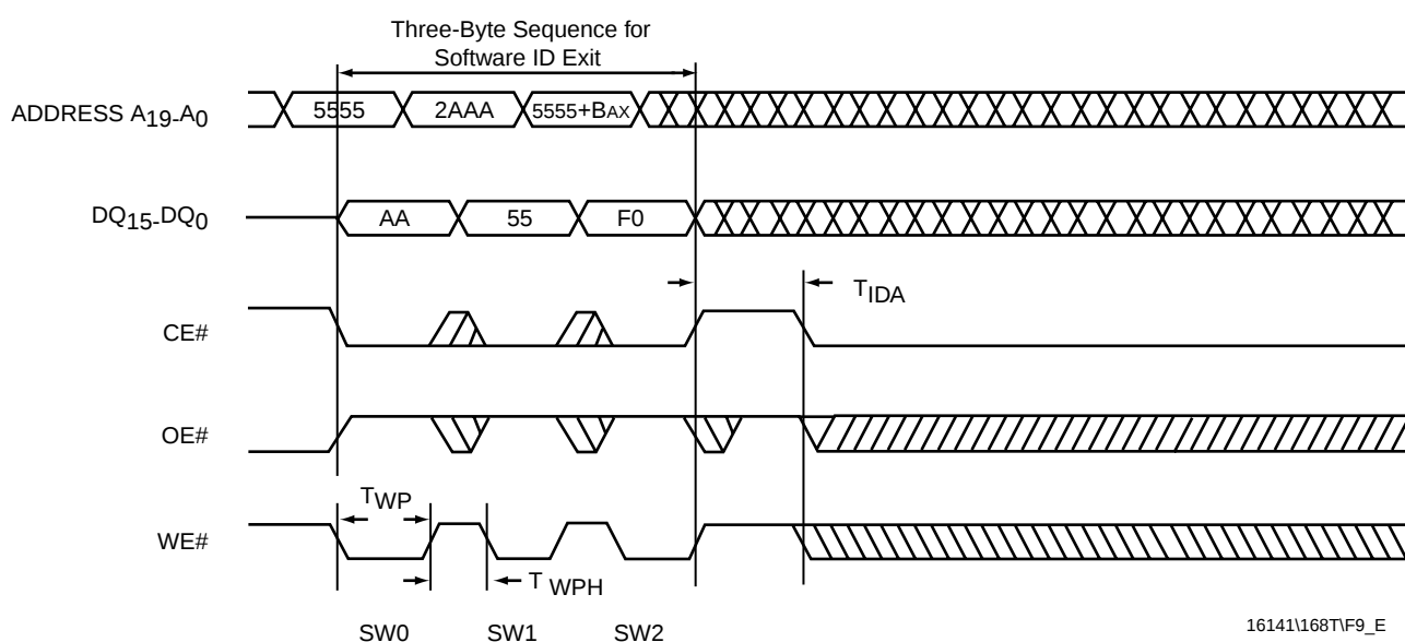
Figure 9: Software ID Exit
