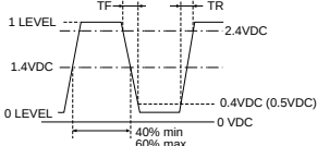
Figure 2) TTL Output Wave Form
