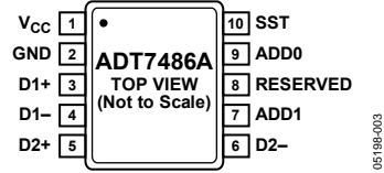
Figure 3. ADT7486A 10-Lead MSOP
