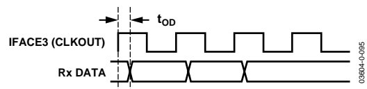
Figure 60. Rx Data Timing Diagram
