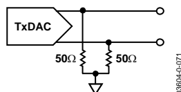
Figure 2. Diagram showing Termination of 100\ \Omega Differential Load for Some TxDAC Measurements
