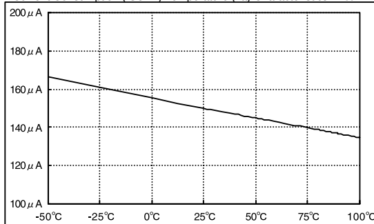
Current Consumption (ISUP3)-Temperature (Ta) Characteristics VCC=14V
