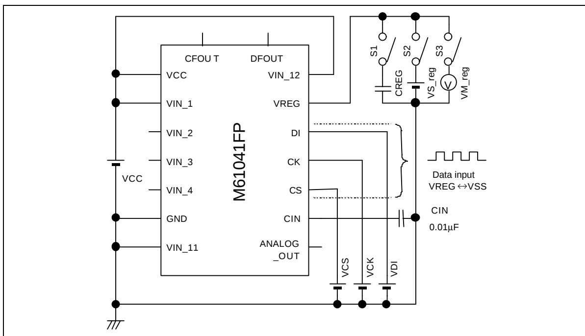
Circuit 2
