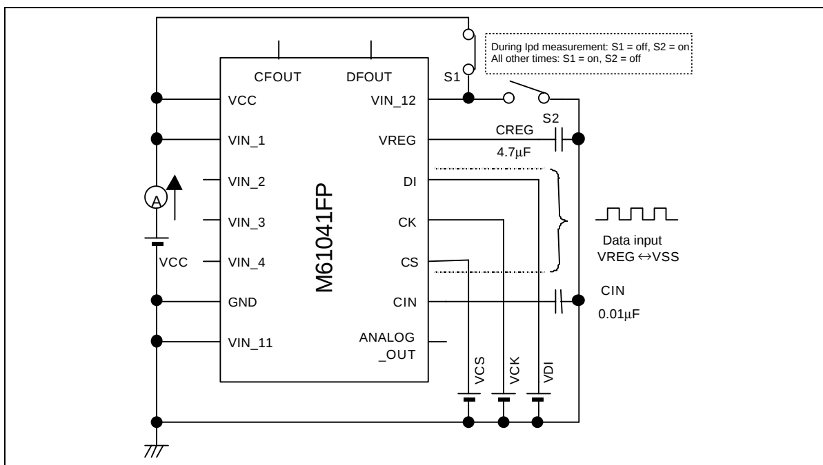
Circuit 1
