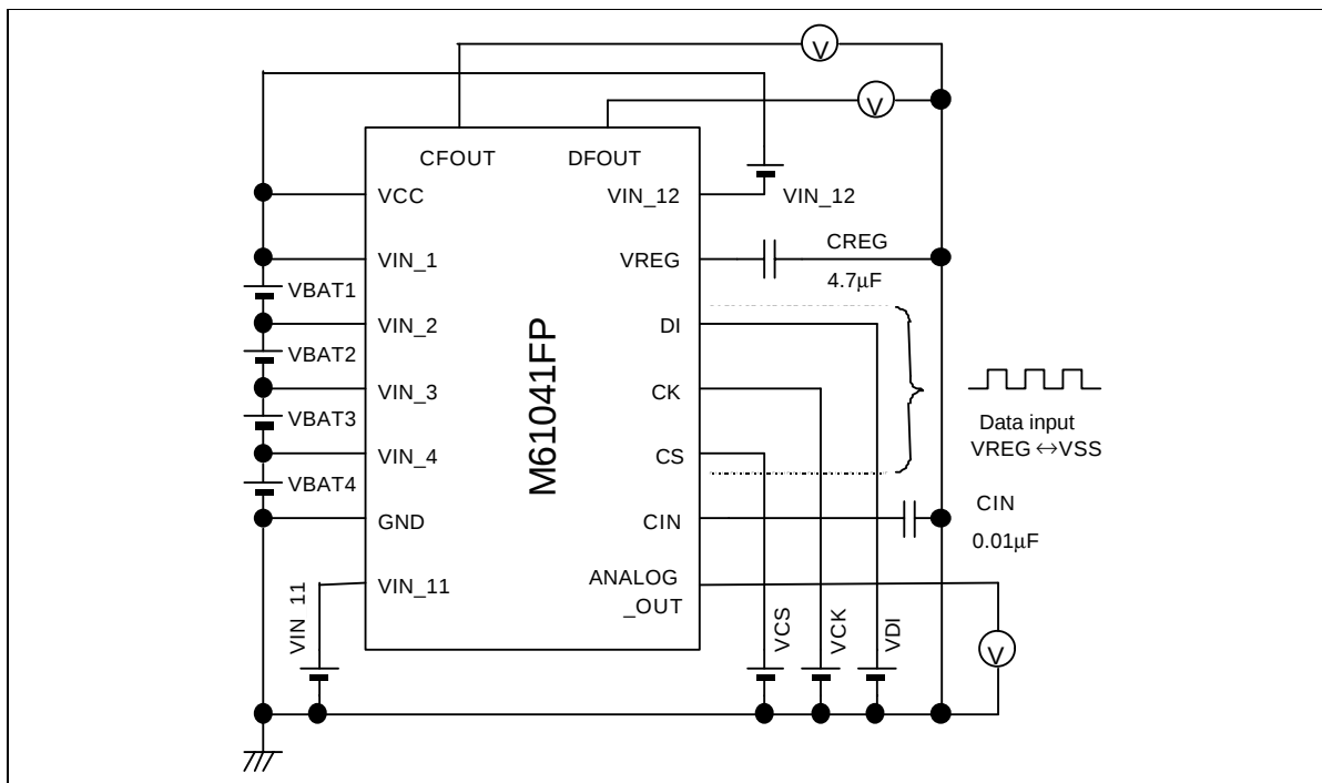
Circuit 9
