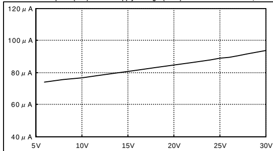
Current Consumption (IPD)-Power Supply Voltage (VCC) Characteristics Temp.=25°C
