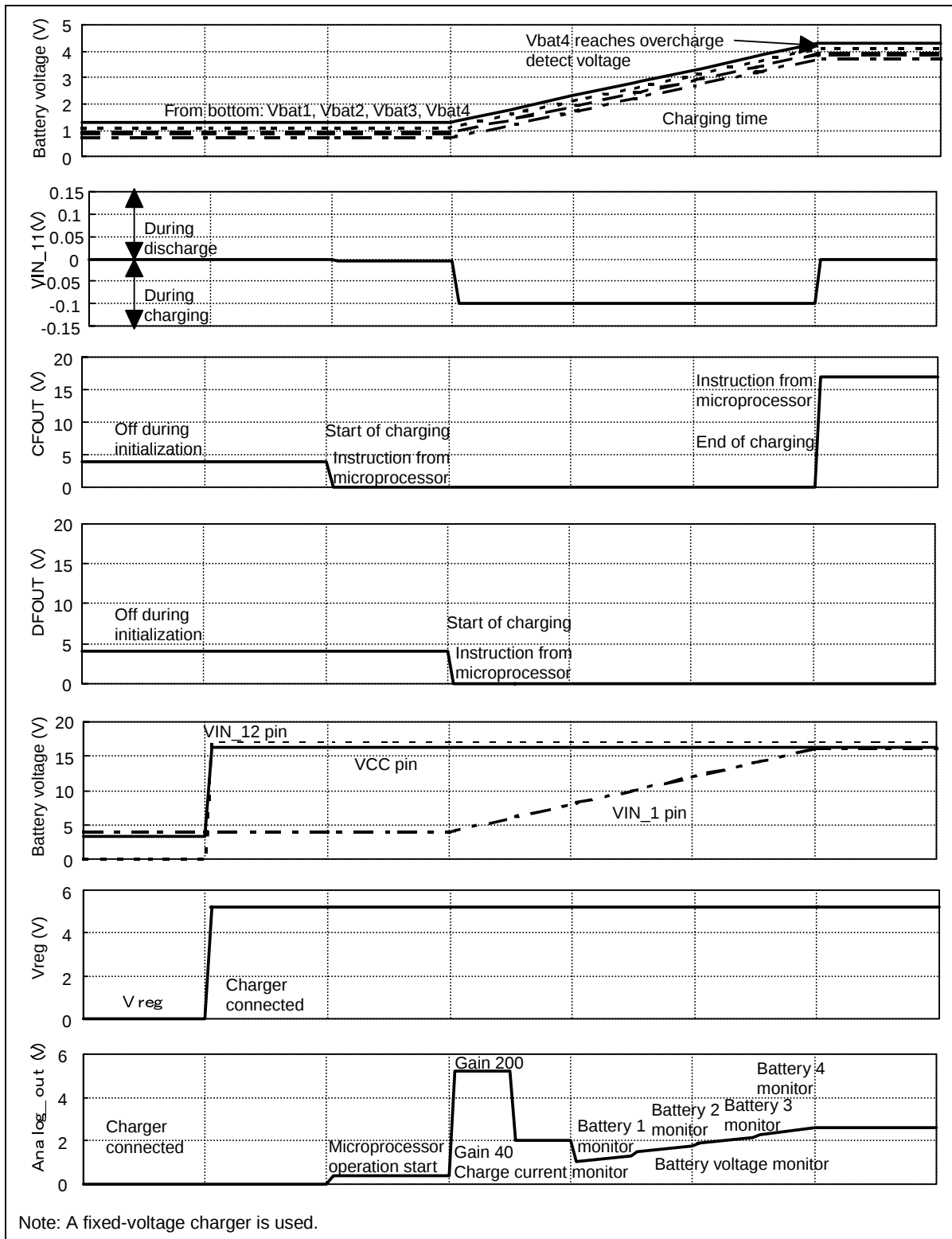
Figure 13 Charging Sequence
