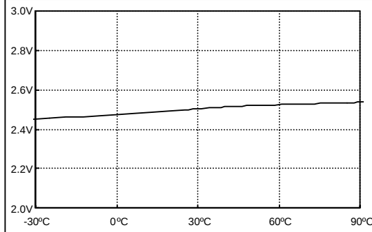
Overcurrent Hold Detect Voltage (VCC-VIOVX)-Temperature (Ta) Characteristics V_{CC}=14V
