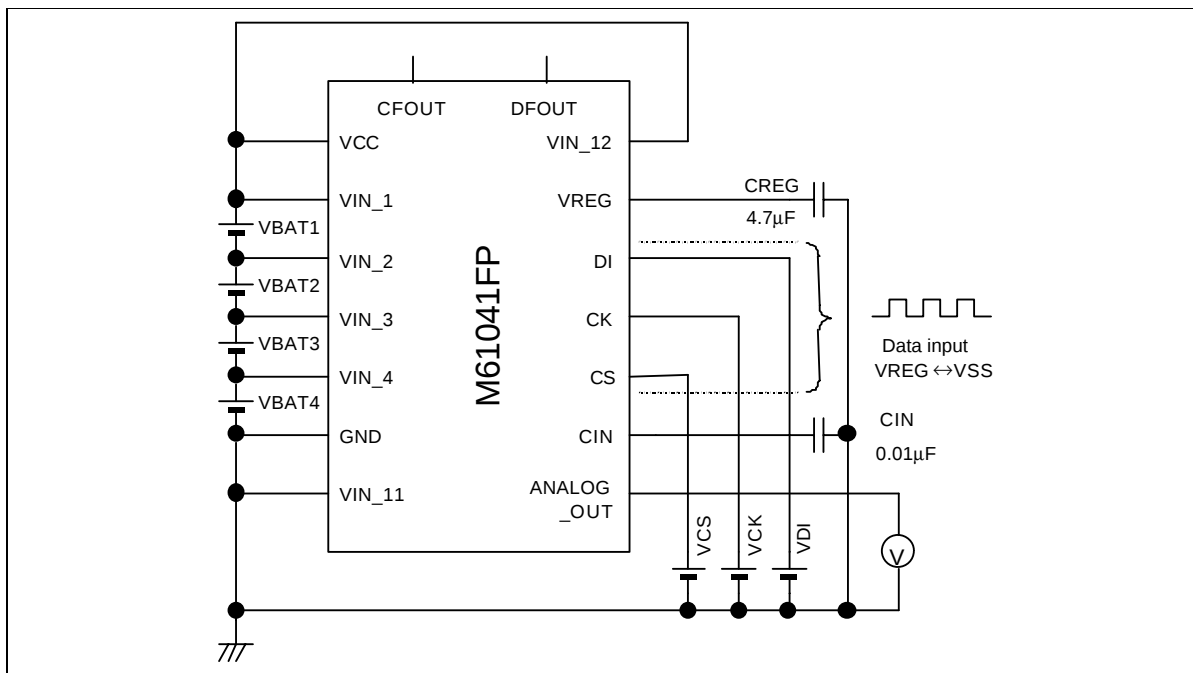
Circuit 5
