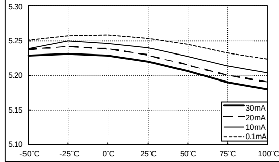
Regulator Output Voltage (VREG)-Temperature (Ta) Characteristics Vcc=14V
