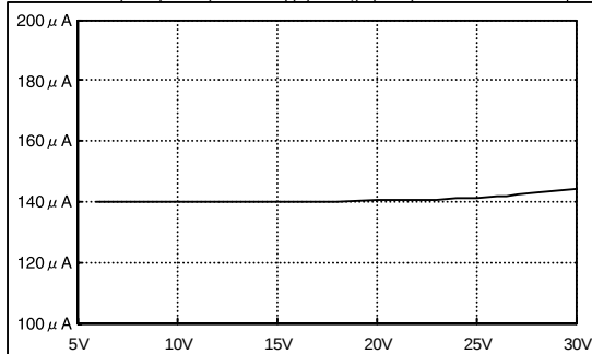
Current Consumption (IPS)-Power Supply Voltage (VCC) Characteristics Temp.=25°C
