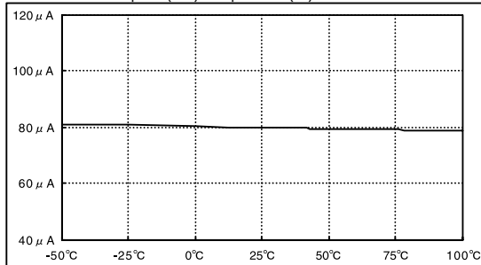
Current Consumption (IPD)-Temperature (Ta) Characteristics VCC=14V
