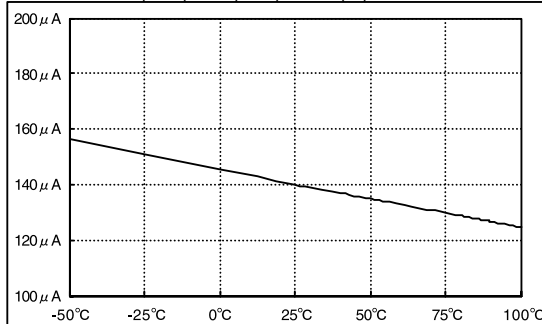
Current Consumption (IPS)-Temperature (Ta) Characteristics VCC=14V
