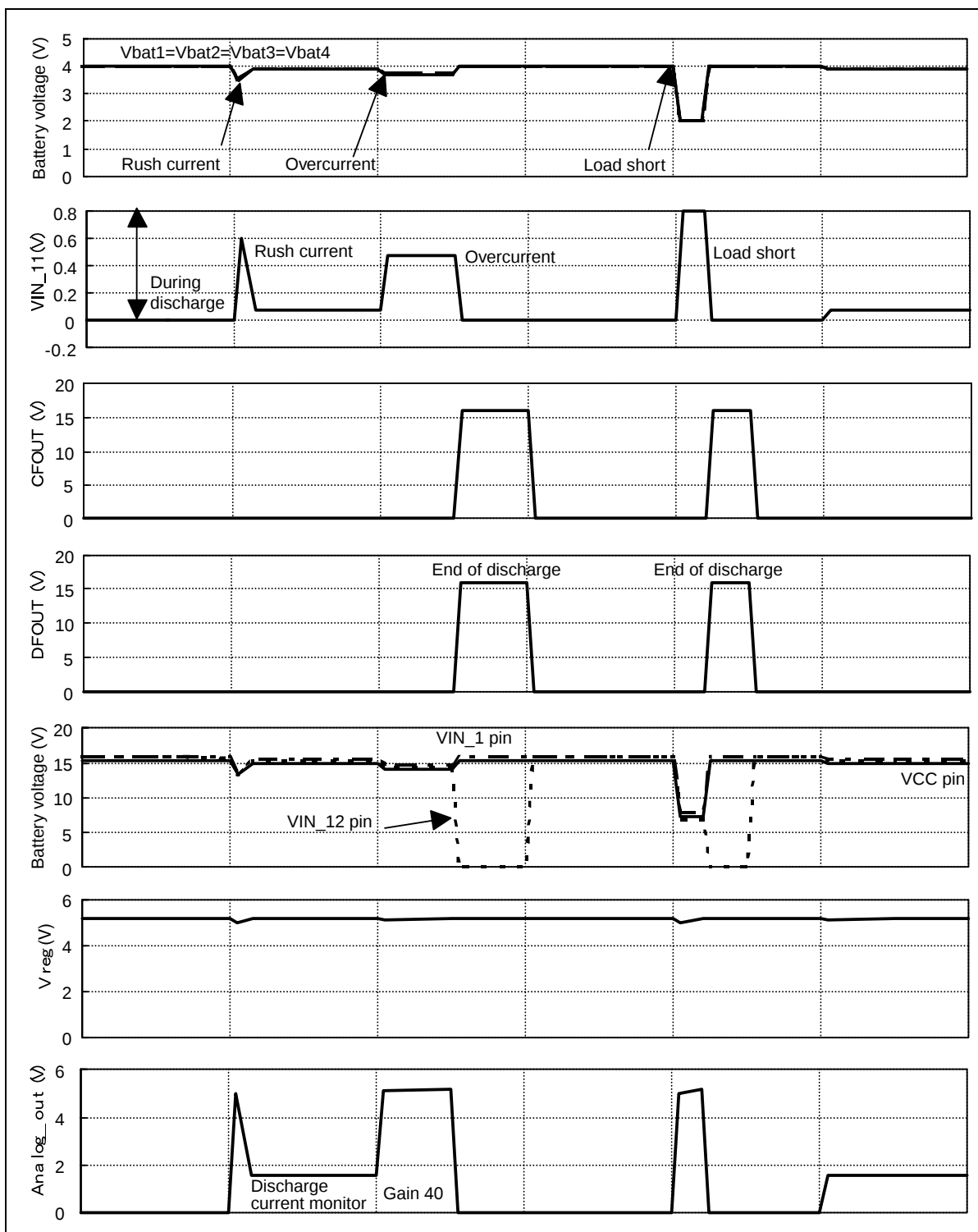
Figure 15 Overcurrent Sequence
