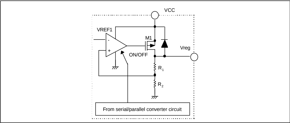
Figure 10 Series Regulator
