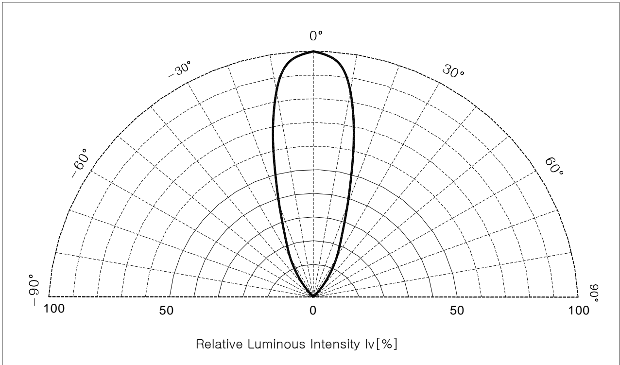
Fig. 5 Radiation Diagram
