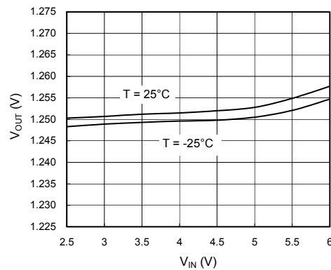
Line Regulation
