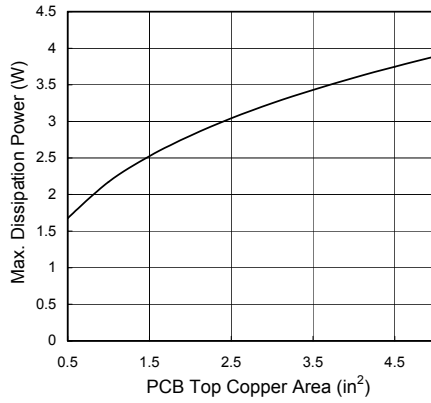
G1084T53(TO-263) Max. Power Dissipation vs. PCB Top Copper Area Area T_{AMB} = 25^{\circ}C ; Still Air
