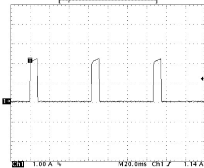
Short Circuit-Current
