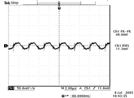
48 Vdc input, 3.3 Vdc/70 A output
