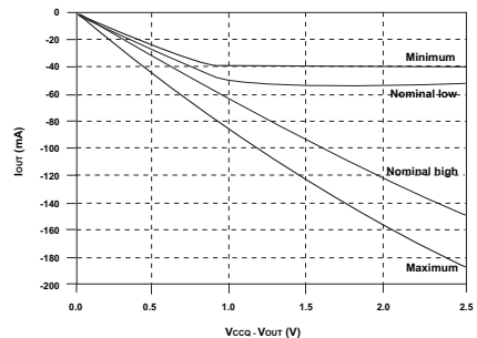
FIGURE B FULL DRIVE PULL-UP CHARACTERISTICS
