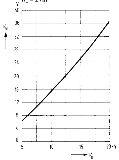
Output voltage versus supply voltage
