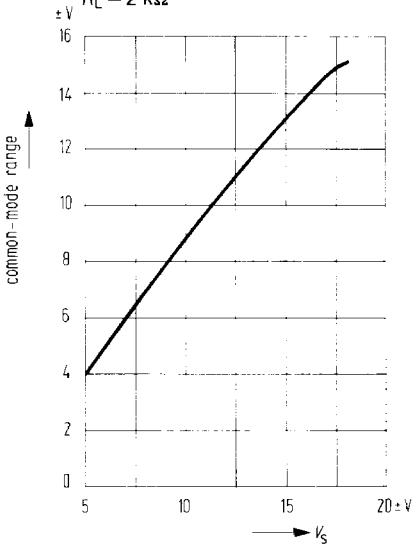
Common-mode range versus supply voltage
