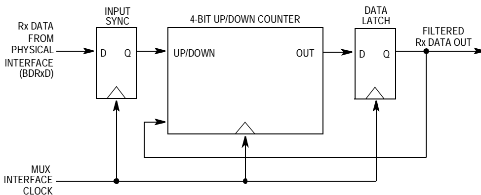
Figure 21-5. BDLC Rx Digital Filter Block Diagram
