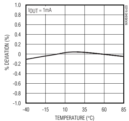
MAX8840 OUTPUT VOLTAGE ACCURACY vs. TEMPERATURE
