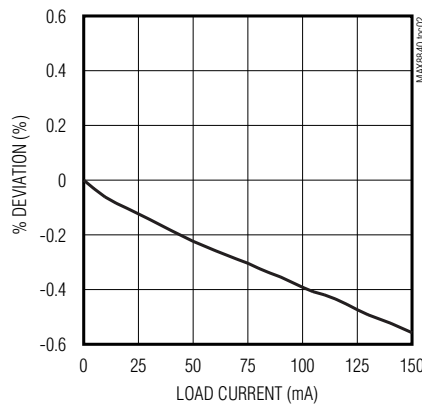
MAX8840 OUTPUT VOLTAGE ACCURACY vs. LOAD CURRENT
