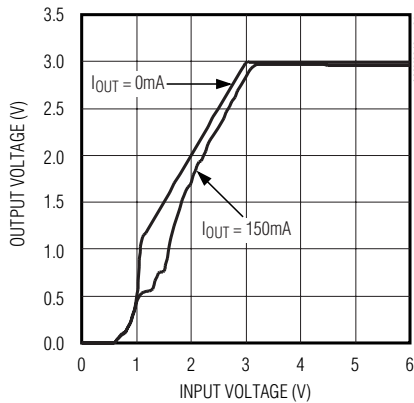
MAX8840 OUTPUT VOLTAGE vs. INPUT VOLTAGE
