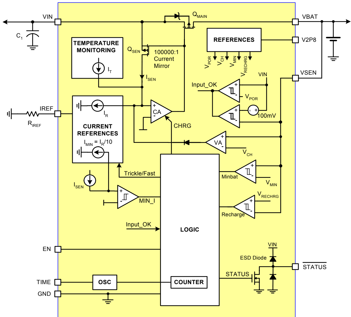
FIGURE 16. BLOCK DIAGRAM
