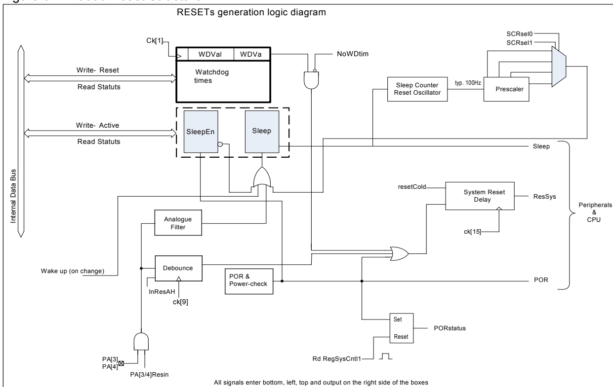
Figure 6. EM6680 Reset Structure
