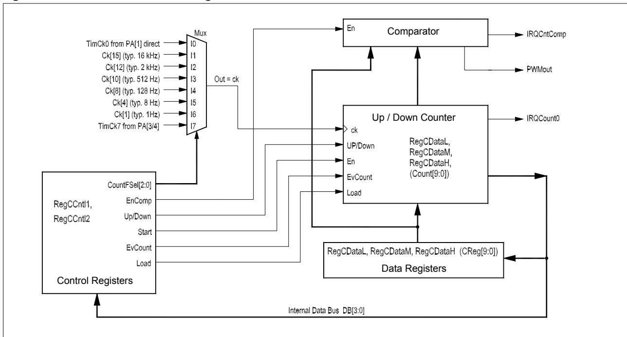
Figure 18. 10-bit Counter Block Diagram
