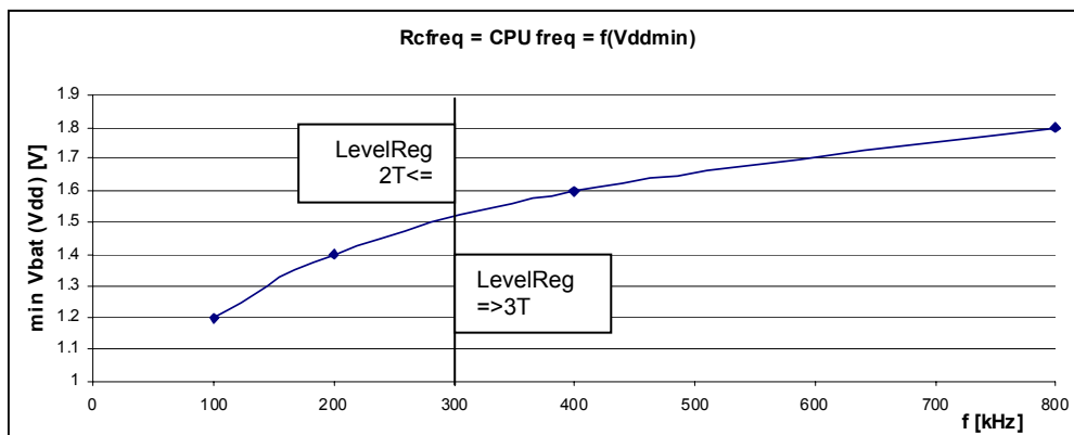
Figure 29. Minimum V_{DD} = f(\text{RC oscillator})
