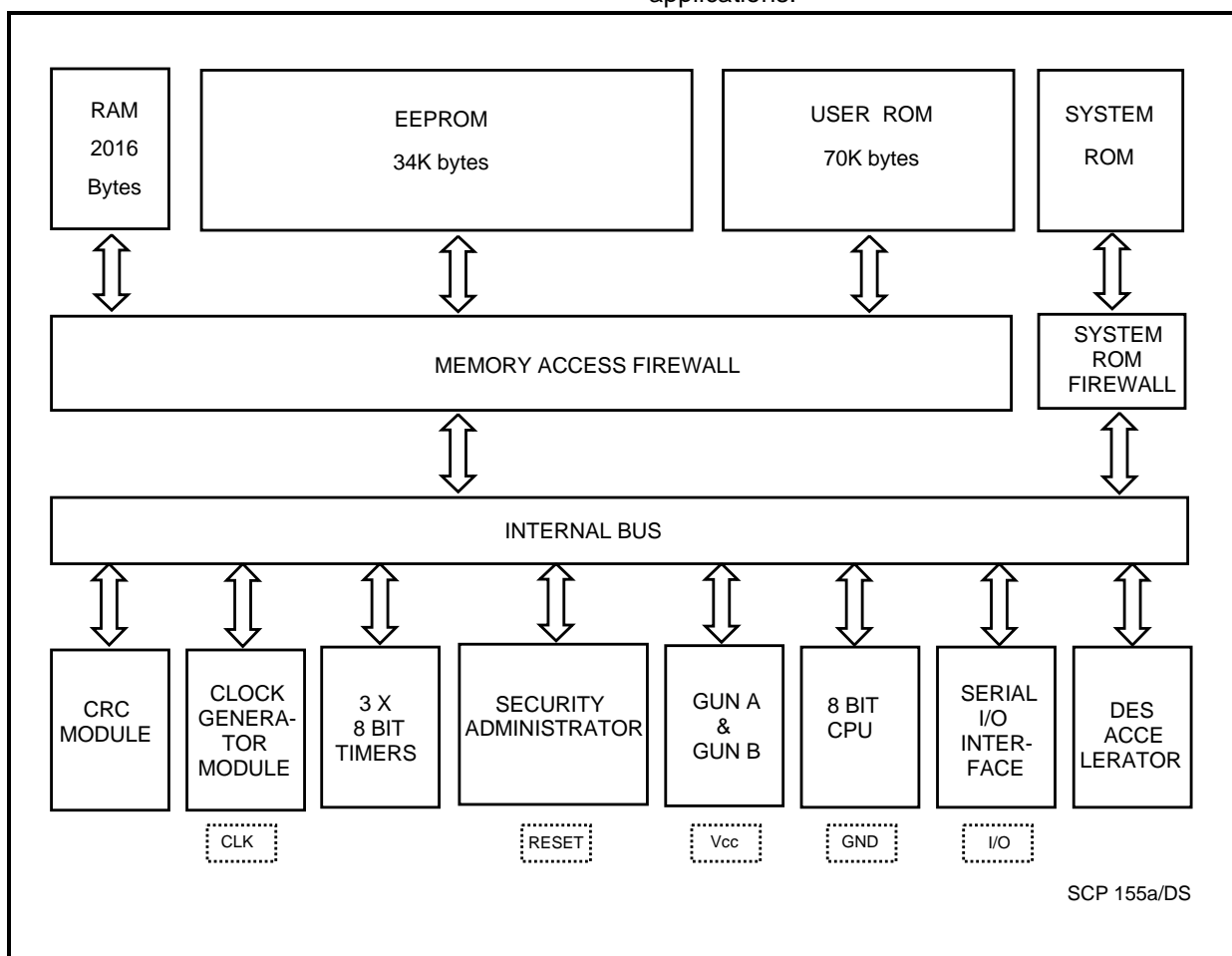
Figure 2 Block diagram
