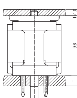
MATING WITH
