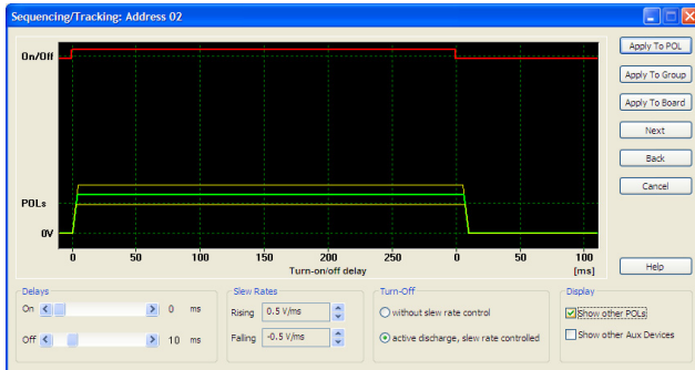
Figure 32. Sequencing/Tracking Window
