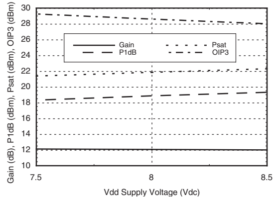
Gain, Power & OIP3 vs. Supply Voltage @ 10 GHz, Fixed Vgg
