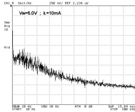
Output Noise
