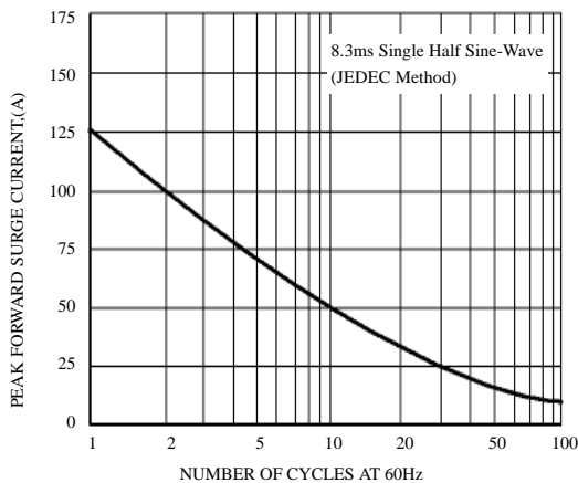
FIG. 5 – MAXIMUM NON-REPETITIVE FOWARD SURGE CURRENT
