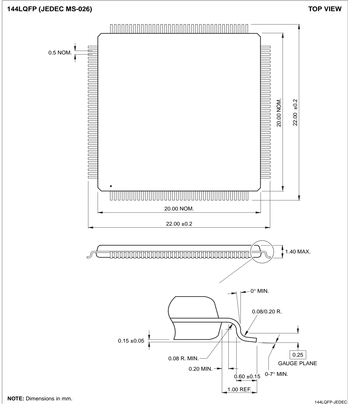
Figure 20. 144-pin LQFP
