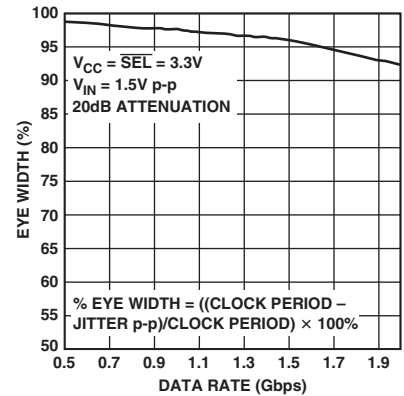
TPC 18. Eye Width vs. Data Rate; PRBS 31
