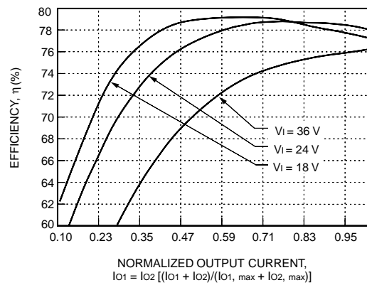
Figure 21. LC010AJ, BK, CL Typical Efficiency vs. Normalized Output Current at Tc = 25 °C
