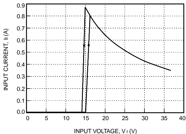
Figure 1. LC010 Input Current vs. Input Voltage at I_o = I_{o, max} and T_c = 25\text{ }^\circ\text{C}
