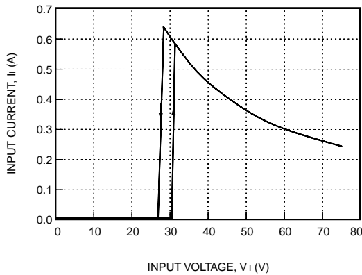
Figure 4. LW015 Input Current vs. Input Voltage at I_{o1} = I_{o, max} and T_c = 25^\circ C
