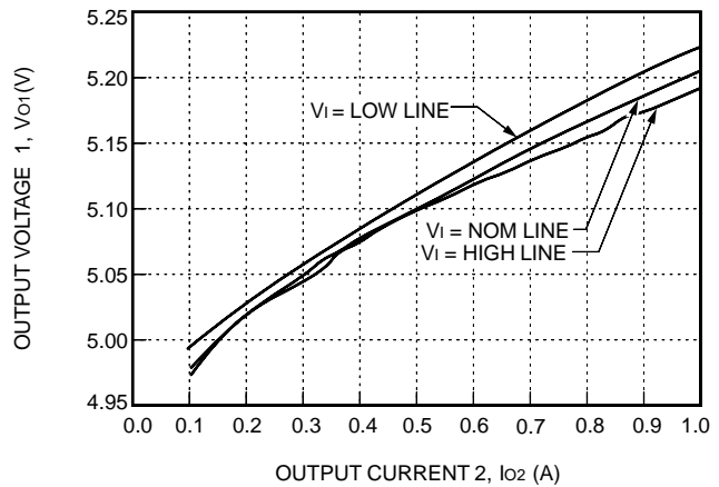
Figure 6. Lx010AJ Typical Load Regulation of Output1 with Fixed I_{o2} = 0.5 A at T_c = 25^\circ C
