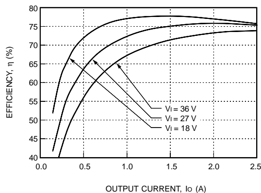
Figure 20. LC010F Typical Efficiency vs. Output Current at Tc = 25 °C
