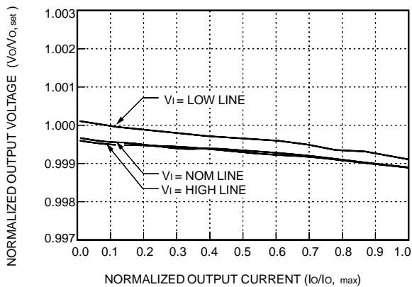
Figure 5. Lx010x/Lx015x Single-Output Load Regulation, Normalized Output Voltage vs. Normalized Output Current at T_c = 25^\circ C
