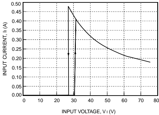
Figure 3. LW010 Input Current vs. Input Voltage at I_{o1} = I_{o, max} and T_c = 25^\circ C
