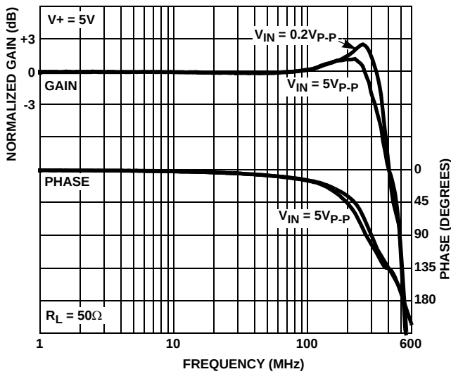
FIGURE 13. FREQUENCY RESPONSE
