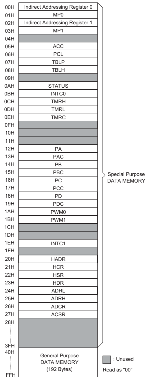
RAM Mapping
