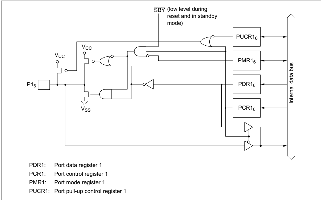
Figure C.1(b) Port 1 Block Diagram (Pin P1 6 )
