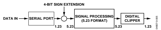
Figure 30. Numeric Precision and Clipping Structure
