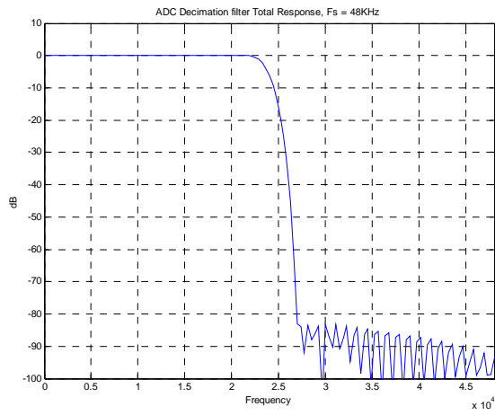
Figure 3. ADC Stopband Filter Response, f_s=48 kHz
