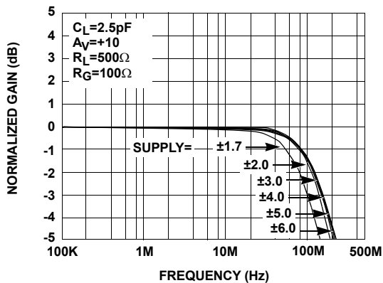
FIGURE 11. GAIN vs FREQUENCY FOR VARIOUS V_{S+} , V_{S-}
