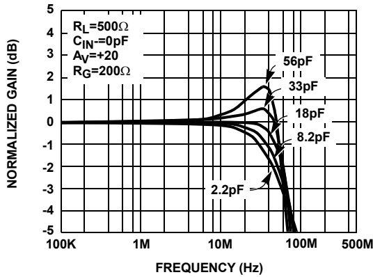
FIGURE 3. GAIN vs FREQUENCY FOR VARIOUS C_L
