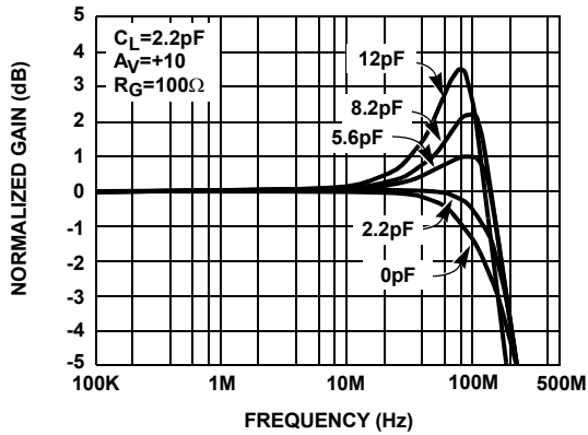
FIGURE 9. GAIN vs FREQUENCY FOR VARIOUS C_{IN}
