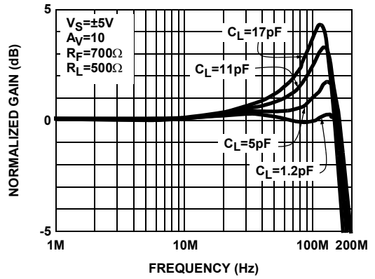
FIGURE 12. NON-INVERTING FREQUENCY RESPONSE FOR VARIOUS C_L
