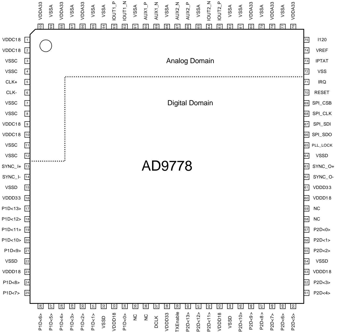
Figure 2. Pin Configuration
