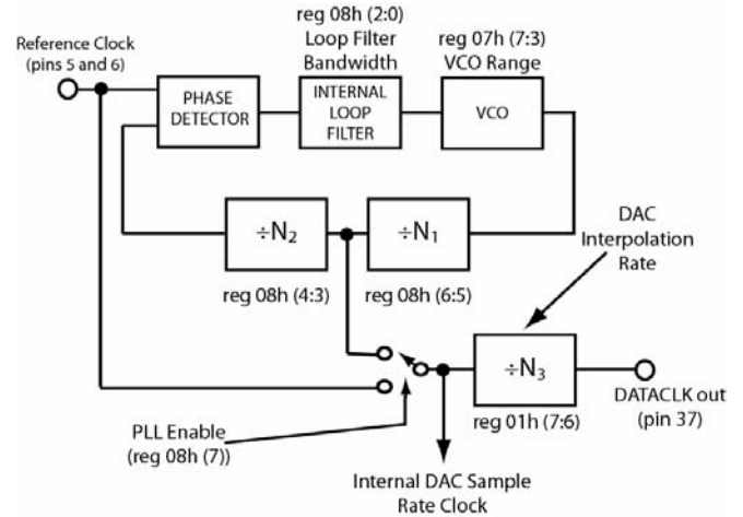
Figure 32. Internal Clock Architecture of AD9778
